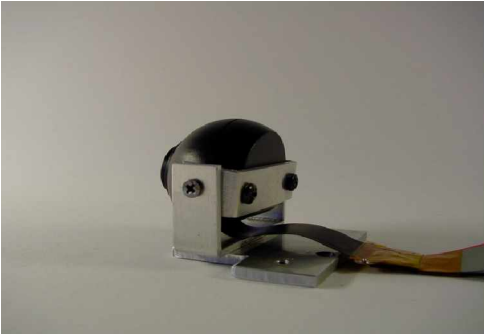
Special holder for original camera head, fixable cameraposition
