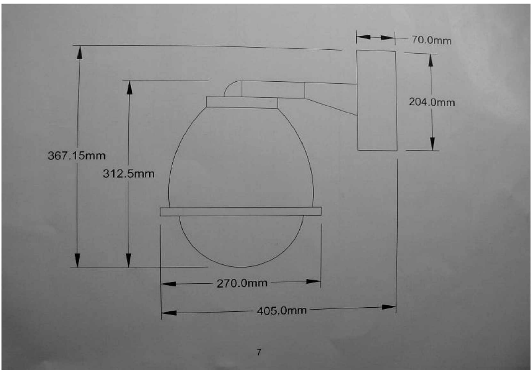
Wall Mounting
